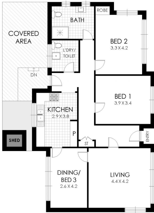
FLOOR PLAN
