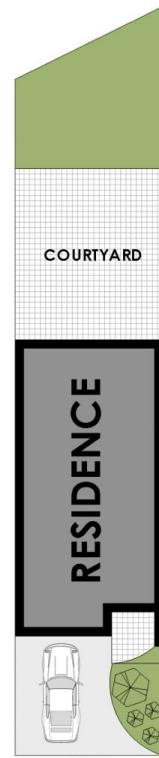
DRIVEWAY SITE PLAN
