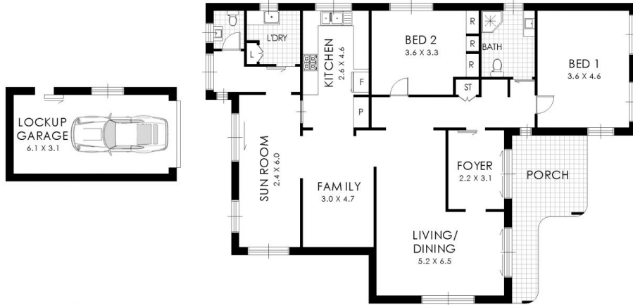
FLOOR PLAN
