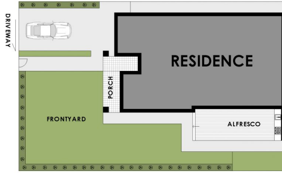
SITE PLAN
