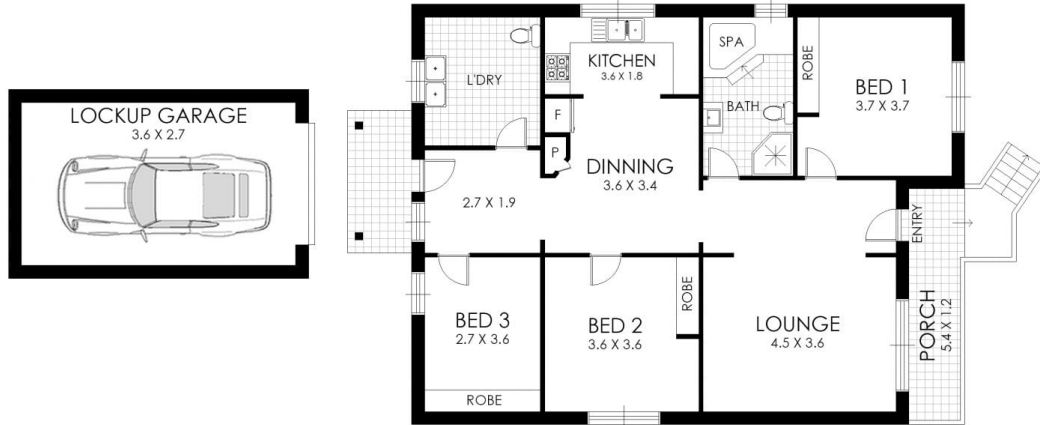
FLOOR PLAN
