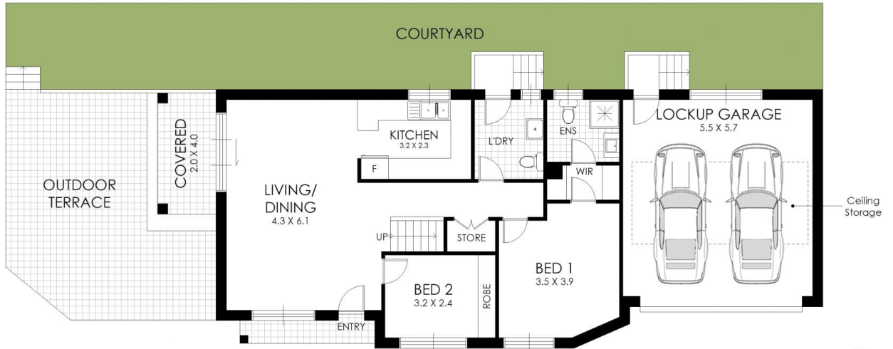
GROUND LEVEL
