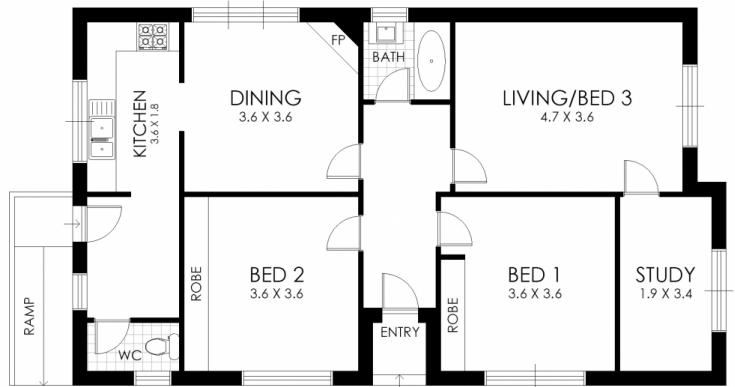
FLOOR PLAN
