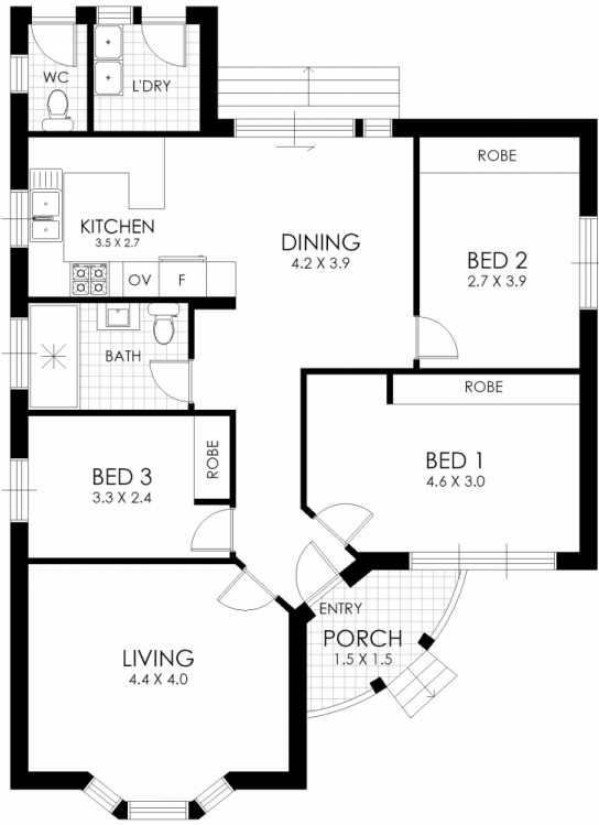
FLOOR PLAN
